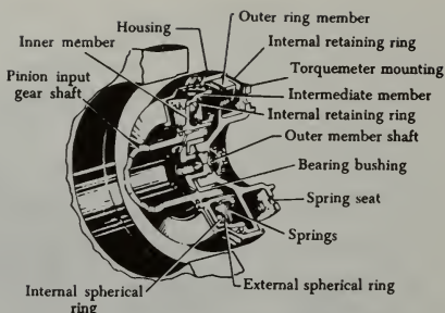
FIGURE 7-32. Safety coupling.
